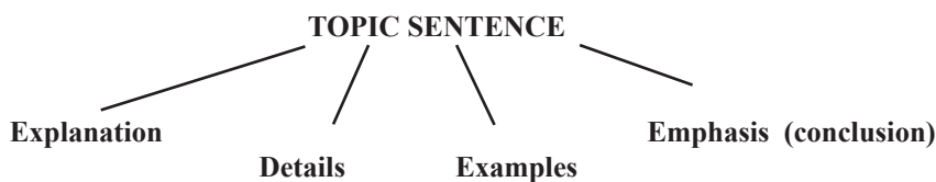
Figure 2: Paragraph structure
